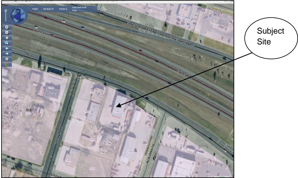
Figure 1. Zoning Map
