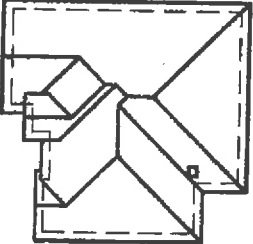
ROOF PLAN SC 1/8" = 1'-0"
