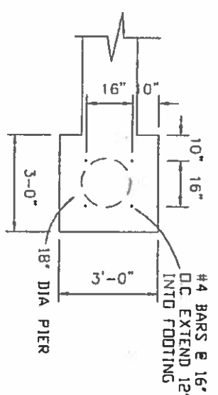
D COLUMN FOUNDATION & DOWEL PLAN 1'-4"=1'
