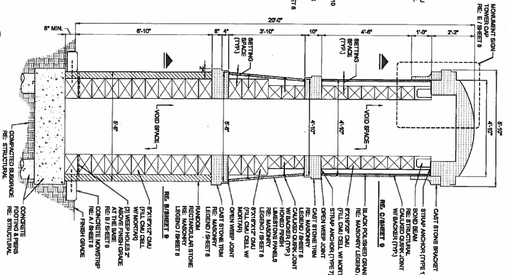
A MONUMENT SIGN TOWER SECTION SCALE: 3/8" = 1'-0"
