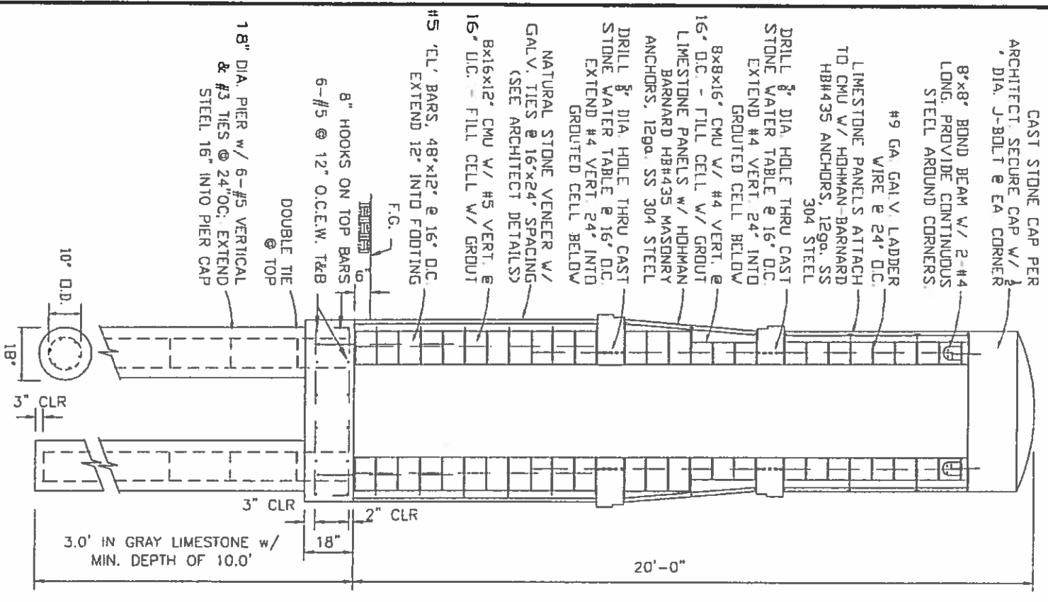
A TOWER SECTION 1'-4"=1'
